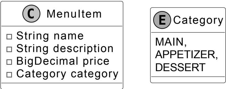
MenuItem class and Category enum
