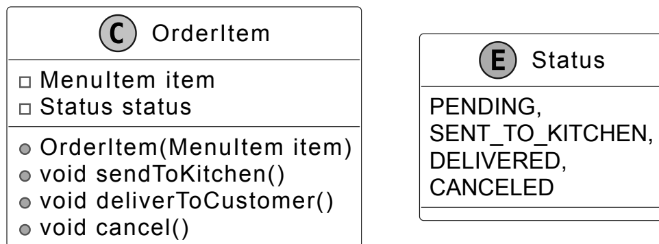
OrderItem class and Status enum
