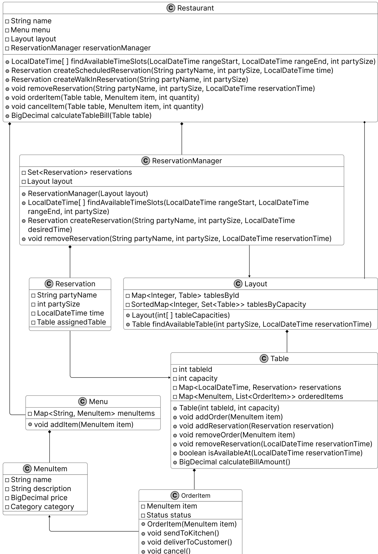
Class Diagram of Restaurant Management System
